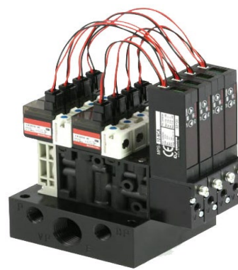
Vacuum ejector unit KMC42
