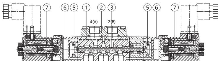
5(R1) 1(P) 3(R2) 5/3 Way H/I/J (Direct mounting)
