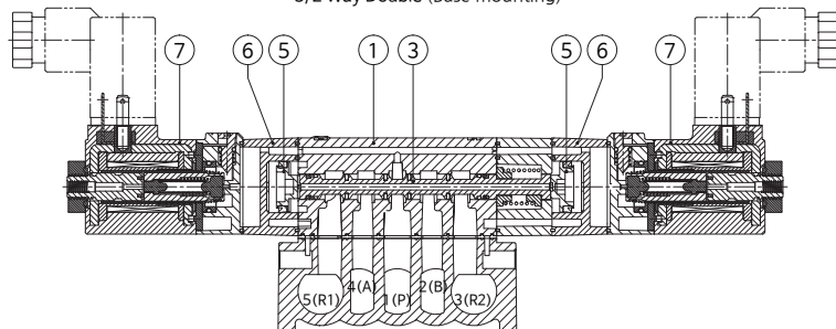
5(R1) 4(A) 1(P) 2(B) 3(R2) 5/3 Way H/I/J (Base mounting)
