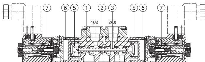
5(R1) 1(P) 3(R2) 5/2 Way Double (Direct mounting)
