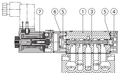
5(R1) 4(A) 1(P) 2(B) 3(R2) 5/2 Way Single (Base mounting)
